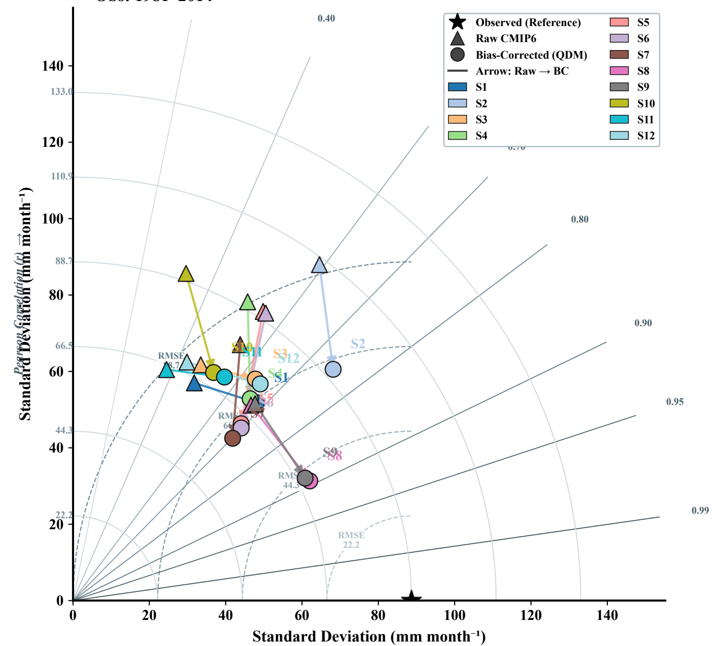
(b) Taylor Diagram — Monthly Scale Obs: 1981–2014
