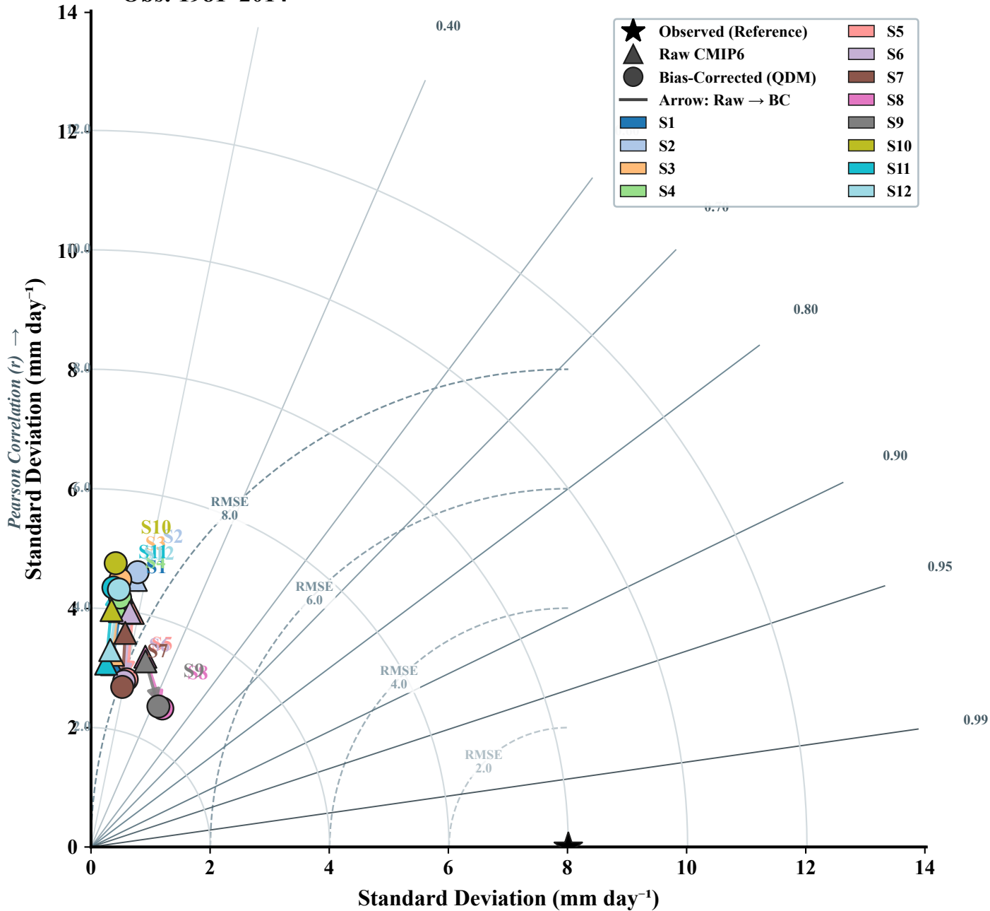
(a) Taylor Diagram — Daily Scale Obs: 1981–2014
